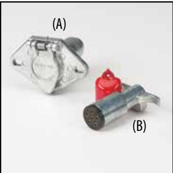
6 WIRE TRAILER PLUG – Female (A) Part No. – EC2020
