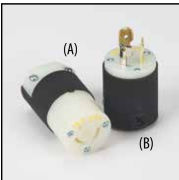
TWIST LOCK CORD CONNECTORS – Female Fits: Hurricane HT-400, HT-500, HT-600, HT-755 & HT-828 (A) Part No. – EC2215 TWIST LOCK CORD CONNECTORS – Male Fits: Hurricane HT-400, HT-500, HT-600, HT-755 & HT-828 (B) Part No. – EC2216
