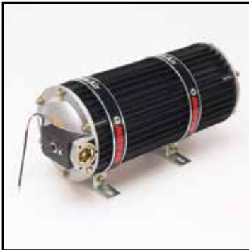
AIR DRYER for Hurricane 1998-2006 w/Fins Fits: Hurricane HT-500, HT-600, HT-755, HT-828 & Vecloader Part No. – AR4011
