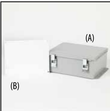
8" x 10" ELECTRICAL BOX Hurricane Baghouse Fits: Hurricane HT-400, HT-500, HT-600, HT-755, HT-828, HS-500 EM, & Quiet Cube Models (A) Part No. – EC2204A 8" x 10" ELECTRICAL BOX INTERIOR PANEL for EC2204A (B) Part No. – EC2204A-1
