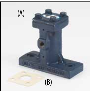
IMPACTING CONE VIBRATOR Fits: Hurricane HT-500, HT-600, HT-755, HT-828, HS-500 EM, HS-800 EM, Quiet Cube & Vecloader (A) Part No. – AR4010
