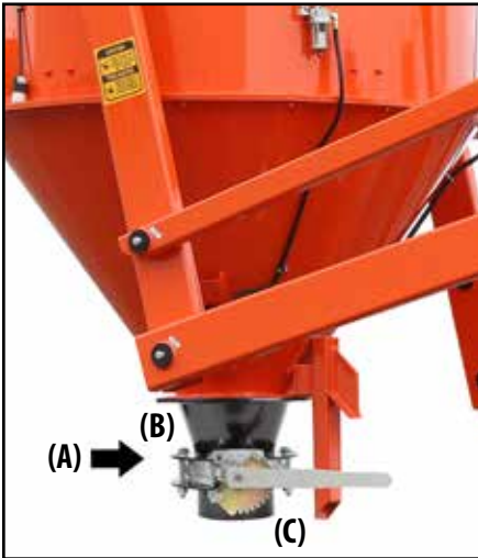
8" SURE SEAL VALVE to Vacuum Cone, Includes: 12" Flange to 8" Flange Reducer Cone (FAB5001) 8" Valve (MC9716) Handle (MC9716-1) 2-8" Flanges, Welded & Assembled (A)Part No. – MC9716-2
