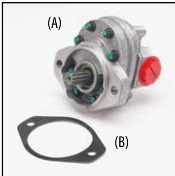
HYDRAULIC PUMP for Auxiliary Drive Engines Fits: Hurricane HT-400, HT-500, HT-600, HT-755 & HT-828 (A) Part No. – HY3008 GASKET – Between HYD Pump and Air Compressor Fits: Hurricane HT-400, HT-500, HT-600, HT-755 & HT-828 (B) Part No. – HY3008-1
