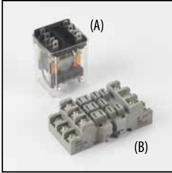
12V RELAY – Vibrator or Asbestos Controls Fits: Vecloder (A) Part No. – EC2010 RELAY SOCKET for EC2010 Fits: Vecloder (B) Part No. – EC2011
