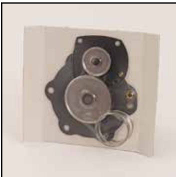
DIAPHRAGM REBUILD KIT For Filter Pulsing on IVEC 20,000 CFM Diesel Dust Collector Part No. – AR4017-3
