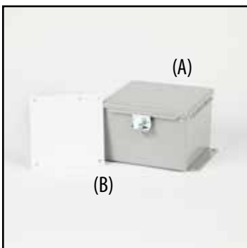
6x6 JIC BOX WITH HINGE FOR HURRICANES WITH AIR CANNON Fits: Hurricane HT-500, HT-600, HS-500 EM & QC-150 (A) Part No. – EC2205A 6x6 JIC BOX INNER PANEL for EC2205A (B) Part No. – EC2205-1
